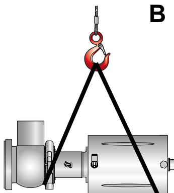
DN80 and DN100 Weight between 25 kg and 50 kg
